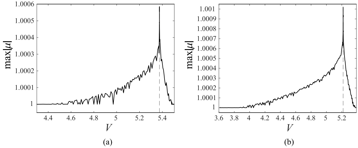
Fig. 15. Maximum modulus of Floquet multipliers for solitary waves in the discrete problem with cubic nonlinearity (4): (a) w_+ = 1 ; (b) w_+ = 6 . Here a = -1 , b = 10 , and the dashed vertical lines mark corresponding superkink velocity values.
