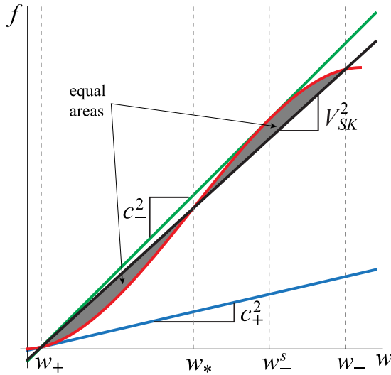
Fig. 1. Interaction force f(w) (red) and the Rayleigh line (black) connecting (w_+, f(w_+)) and (w_-, f(w_-)) (black). The strain w_* marks the transition from the hardening (convex) to softening (concave) regime. A superkink transition wave with limiting states w_\pm and supersonic velocity V_{SK} such that V_{SK}^2 > f'(w_\pm) exists when the two shaded areas cut by the Rayleigh line, which has the slope V^2 , are equal. The associated solitary wave solutions have velocity V such that either c_+^2 < V^2 < V_{SK}^2 or V_{SK}^2 < V^2 < c_-^2 , where c_+^2 and c_-^2 are the slopes of the blue and green straight lines passing through (w_+, f(w_+)) and tangent to f(w) at w_+ and w_-^s , respectively. See the text for more details.
