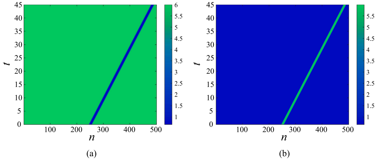
Fig. 16. Space-time strain evolution initiated by computed solitary wave solutions slightly below and slightly above the superkink limit, with velocities (a) V = 5.21749194749 (a compressive wave); (b) V = 5.2174919476 (a tensile wave). Here a = -1 , b = 10 , w_+ = 6 , V_{SK} = 7\sqrt{5}/3 = 5.21749194749951 .
