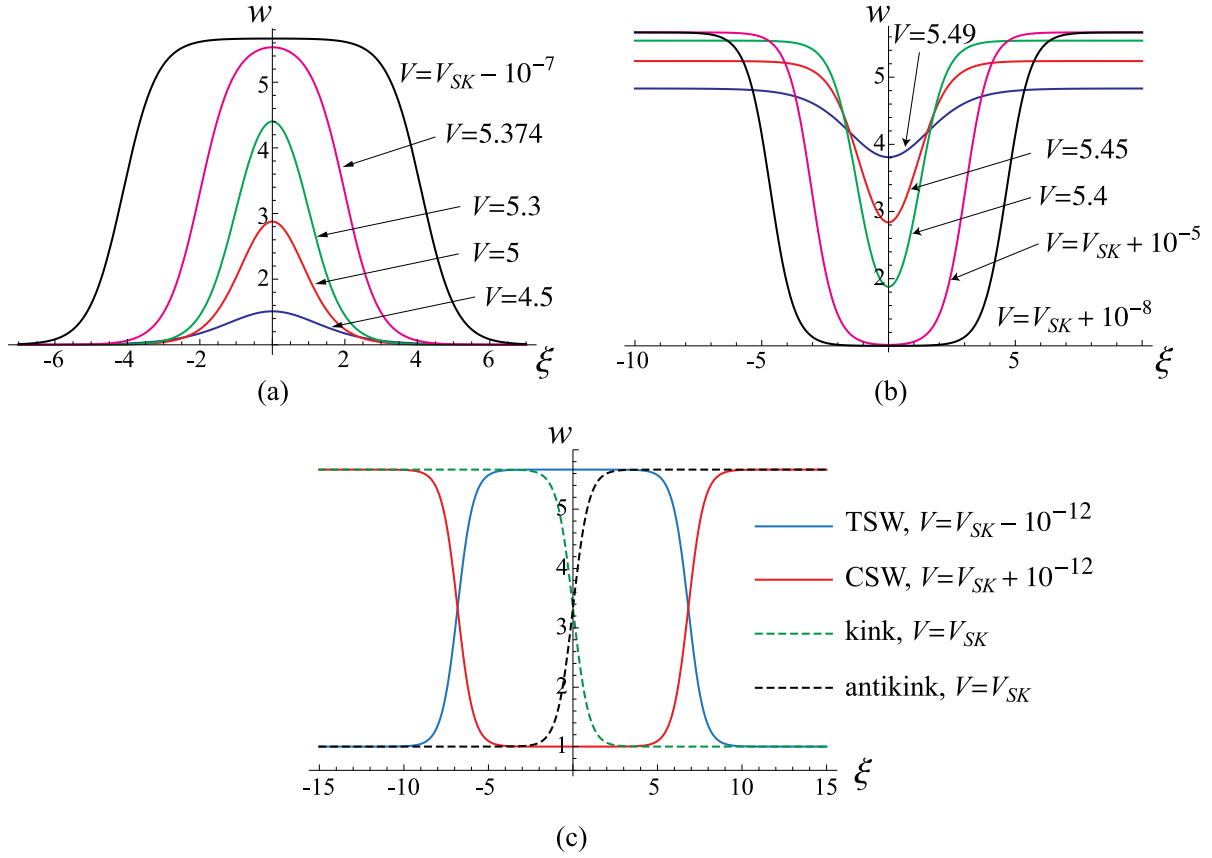
Fig. 5. (a) Tensile solitary waves (TSW) in the QC model with cubic nonlinearity (4) at c_+ < V < V_{SK} ; (b) compressive solitary waves (CSW) at V_{SK} < V < c_- ; (c) solitary waves just below and just above V_{SK} , shown together with kink and antikink fronts. Here w_+ = 1 , a = -1 , b = 10 , yielding V_{SK} = 2\sqrt{65}/3 , w_- = 17/3 , c_+ = 3\sqrt{2} , c_- = 11/2 .
