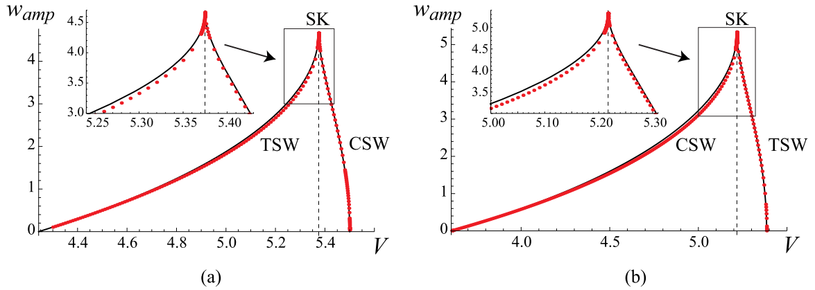
Fig. 9. (a) Amplitude w_{amp} = |w(0) - w_+| as a function of velocity V for solitary wave solutions of the discrete problem (8) (dots) with cubic nonlinearity (4) and the corresponding solutions for the QC model (18) (solid curves): (a) w_+ < w_* ; (b) w_+ > w_* . The superkink limit (SK) is marked by the dashed vertical line, and tensile and compressive waves are marked by TSW and CSW, respectively. Here a = -1 , b = 10 , and the values of w_+ and the corresponding superkink velocity V_{SK} and sonic speeds c_{\pm} are w_+ = 1 , V_{SK} = 2\sqrt{65}/3 , c_+ = 3\sqrt{2} , c_- = 11/2 in (a) and w_+ = 6 , V_{SK} = 7\sqrt{5}/3 , c_+ = \sqrt{13} , c_- = \sqrt{29} in (b). Insets zoom in inside the rectangles.
