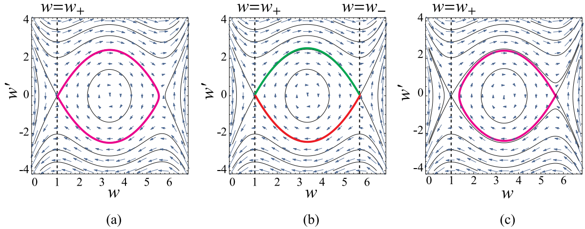
Fig. 2. Phase portraits for (17) with f(w) given by (4), w_+ = 1 and (a) V = V_{SK} - 0.001 ; (b) V = V_{SK} ; (c) V = V_{SK} + 0.005 , where V_{SK} satisfies the conditions (12), (14) with the corresponding w_- . See the text for details. Here V_{SK} = 2\sqrt{65}/3 , w_- = 17/3 . The colored trajectories correspond to a tensile solitary waves in (a), superkinks in (b) and a compressive solitary wave in (c).
