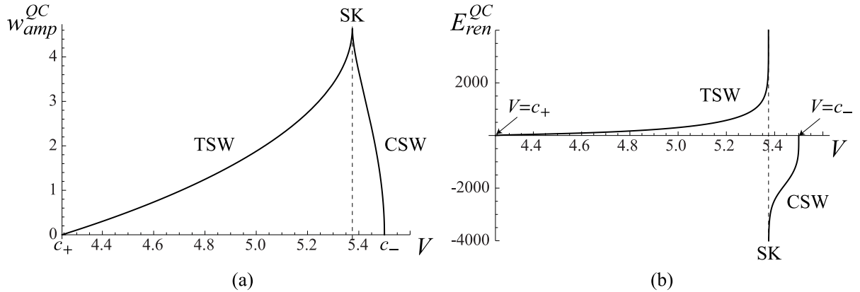
Fig. 6. (a) Amplitude (33) and (b) renormalized energy (34) as functions of velocity V for solitary waves in QC model at w_+ = 1 . Here a = -1 , b = 10 , and the superkink (SK) limit V_{SK} = 2\sqrt{65}/3 is marked by the dashed vertical line. The sonic limits are c_+ = 3\sqrt{2} and c_- = 11/2 .
