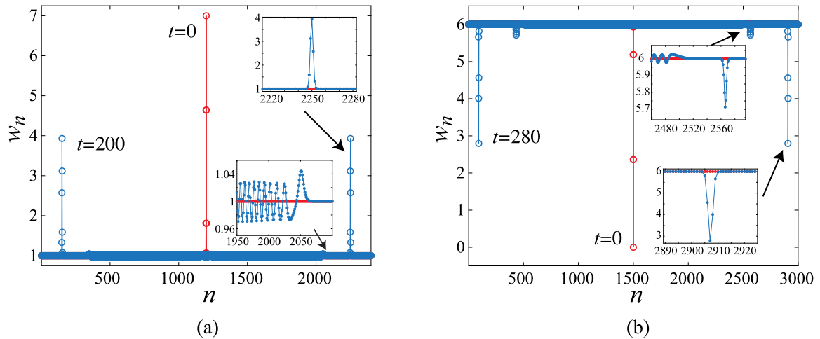
Fig. 17. Initial and final strain profiles in simulations with cubic nonlinearity (4) and initial data (43) with (a) w_B = 1 , A = 6 , L = 2400 ; (b) w_B = 6 , A = -6 , L = 3000 . Insets zoom in on the solitary and dispersive waves. Here a = -1 , b = 10 .
