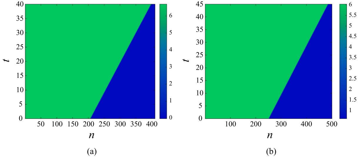
Fig. 13. Space-time strain evolution initiated by computed superkink solutions with velocities (a) V = 4.8 ; (b) V = 5.2 . Here a = -1 , b = 10 .
