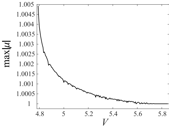
Fig. 11. Maximum modulus of Floquet multipliers for superkink solutions in the discrete problem with cubic nonlinearity (4). Here a = -1 , b = 10 .
