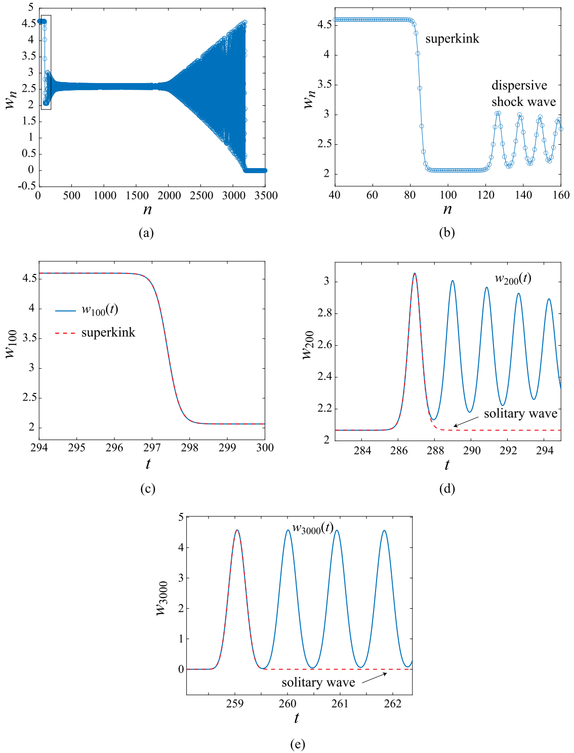
Fig. 14. The results of simulations with Riemann initial data (42) with w^l = 4.6 , w^r = 0 , L = 3600 and cubic nonlinearity (4): (a) strain profile at t = 300 ; (b) enlarged version of the region inside the rectangle in (a); (c) superkink with V = -5.7209 (red dashed curve) and w_{100}(t) (blue curve); (d) solitary wave with V = -5.6159 , w_B = 2.0667 (red dashed curve) and w_{200}(t) (blue curve); (e) solitary wave with V = 4.6404 , w_B = 0 (red dashed curve) and w_{3000}(t) (blue curve). Here a = -1 , b = 10 .
