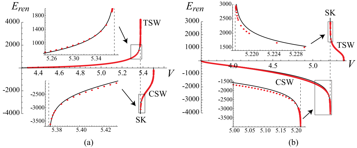
Fig. 10. Renormalized energy E_{ren} given by (39) as a function of velocity V for solitary wave solutions of the discrete problem (8) (dots) with cubic nonlinearity (4) and the corresponding energy (34) for the QC model (18) (solid curves): (a) w_+ < w_* ; (b) w_+ > w_* . The superkink limit (SK) is marked by the dashed vertical line, and tensile and compressive waves are marked by TSW and CSW, respectively. Here a = -1 , b = 10 , and the values of w_+ and the corresponding superkink velocity V_{SK} and sonic speeds c_{\pm} are w_+ = 1 , V_{SK} = 2\sqrt{65}/3 , c_+ = 3\sqrt{2} , c_- = 11/2 in (a) and w_+ = 6 , V_{SK} = 7\sqrt{5}/3 , c_+ = \sqrt{13} , c_- = \sqrt{29} in (b). Insets zoom in inside the rectangles.
