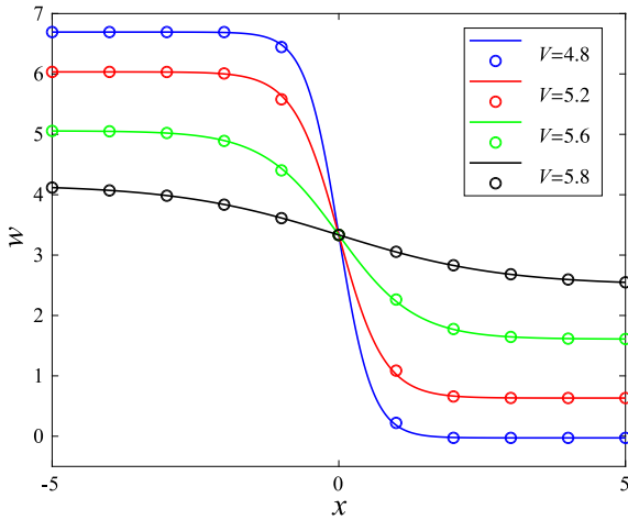
Fig. 7. Superkink solutions w_n(0) = w(n) of the discrete problem (8) (circles) with cubic nonlinearity (4) and the corresponding solutions w(x) for the QC model (18) (solid curves) evaluated at t = 0 . Here a = -1 , b = 10 .
