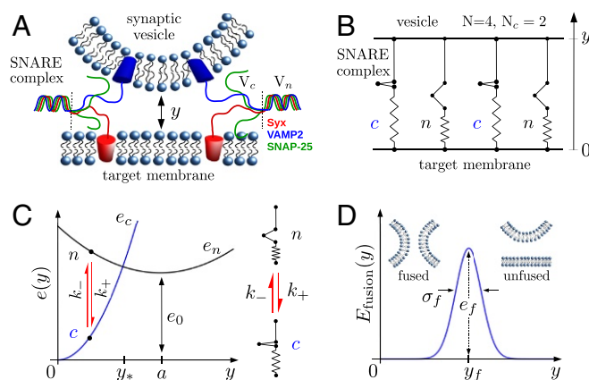
Fig. 1. The fusion machinery. (A) Schematic of the two membranes with two attached SNAREpins. (B) Mechanical model with N=4 SNAREpins in parallel bridging the two membranes separated by the distance y . Two SNAREpins are in state c , and two are in state n ; therefore, N_c = 2 . (C) Model of a single SNAREpin. (D) Fusion energy landscape. Table 1 has the complete list of parameter values.
