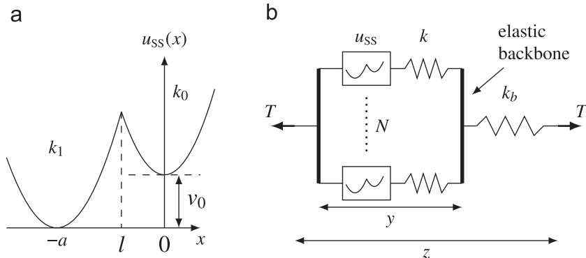
Fig. 7. Snap-spring model of a cluster. (a) Dimensional energy landscape of a bistable crosslinker. (b) Structure of a parallel bundle containing N crosslinkers in a soft device.
