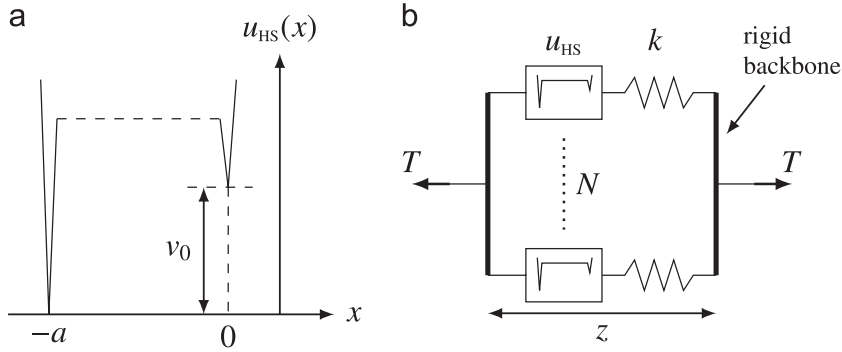
Fig. 1. Hard spin model of a parallel bundle of bistable crosslinkers. (a) Energy landscape of an individual crosslinker; (b) N crosslinkers loaded in a soft device.
