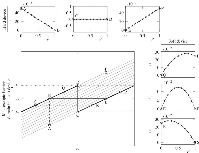
Fig. 6. Summary of the behavior of the HS model. The main frame shows the tension–elongation relations corresponding to p = 0, 0.1, \dots, 1 for a system with N=10 (gray lines) and the tension–elongation relation in the global minimum (thick lines). The horizontal dotted lines show the limit of the domain where a macroscopic energy barrier is present in a soft device. The satellite frames (above, hard device; right, soft device) show the energy barriers corresponding to various transitions ( A \rightarrow B , C \rightarrow D , ...) shown by dashed lines in the main frame.
