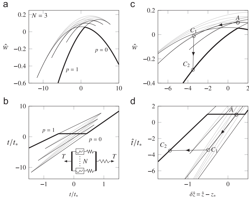
Fig. 10. Mechanical response of the snap-spring model in a soft device. (a) Energy levels of all the (p, r) configurations for the case N=3 at different applied tensions. (b) Corresponding tension–elongation relations. Solid lines, metastable states with p = 0, 1/3, 2/3, 1 and r = 1 - p, q=0 ; dotted lines, unstable states with q \neq 0 ; thick lines, global minimum corresponding to p = 0, r = 1 for t > t_* and to p = 1, r = 0 , for t < t_* . (c,d) zoom in of (a and b) illustrating the response of the system to abrupt shortening with an elastic unloading ( A \rightarrow B_1 ) followed by a massive conformational change in isometric conditions ( C_1 \rightarrow C_2 ). Parameters are as in Fig. 9.
