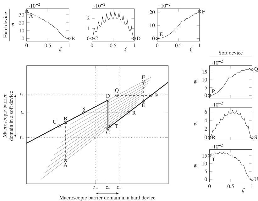
Fig. 13. Overall behavior of the snap-spring model. The main frame shows the tension–elongation relations corresponding to p = 0, 0.1, \dots, 1 , for a system with N=10 (gray lines) and the tension–elongation relations in the global minimum (thick lines). The dotted lines show the limit of the domain where a macroscopic energy barrier is present in a hard device (vertical lines) and in a soft device (horizontal lines). The satellite frames (above, hard device; right, soft device) show the energy barriers corresponding to various transitions shown by dashed lines in the main frame. In particular, the transition C \rightarrow D (hard device) and the transition R \rightarrow S (soft device) correspond to z = z_* and t = t_* , respectively. The other hard device transitions, A \rightarrow B and E \rightarrow F , are outside the bistable interval [z_-, z_+] and thus contain a collective transition. The other soft device transitions, P \rightarrow Q and T \rightarrow U , exhibit the same kind of synchronization along the segment of the ‘reaction path’ which is located inside the bistable domain. Parameters other than N are as in Fig. 9.
