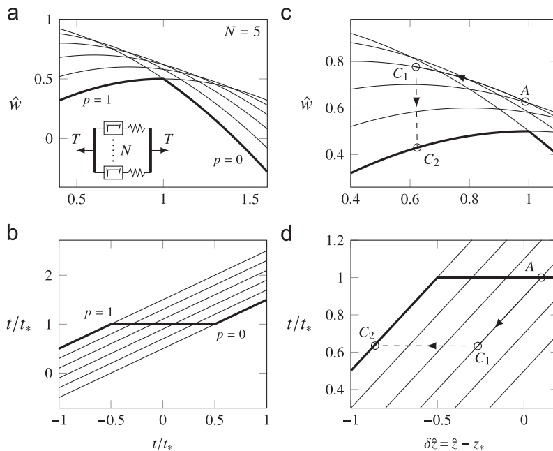
Fig. 4. Mechanical response of the HS model in a soft device. (a) Energy levels of the metastable states ( p = 0, \frac{1}{5}, \dots, 1 ) for different applied forces. (b) Corresponding tension–elongation relations. In (c) and (d) we zoom into domain near t = t_* = v_0 and show schematically the response of the system to a sudden application of a load increment with an elastic phase ( A \rightarrow C_1 ) followed by a folding phase C_1 \rightarrow C_2 . Thick lines, global minimum corresponding to p=0 ( p=1 ) for t > t_* ( t < t_* ). Parameters are v_0 = 1 and N=5 .
