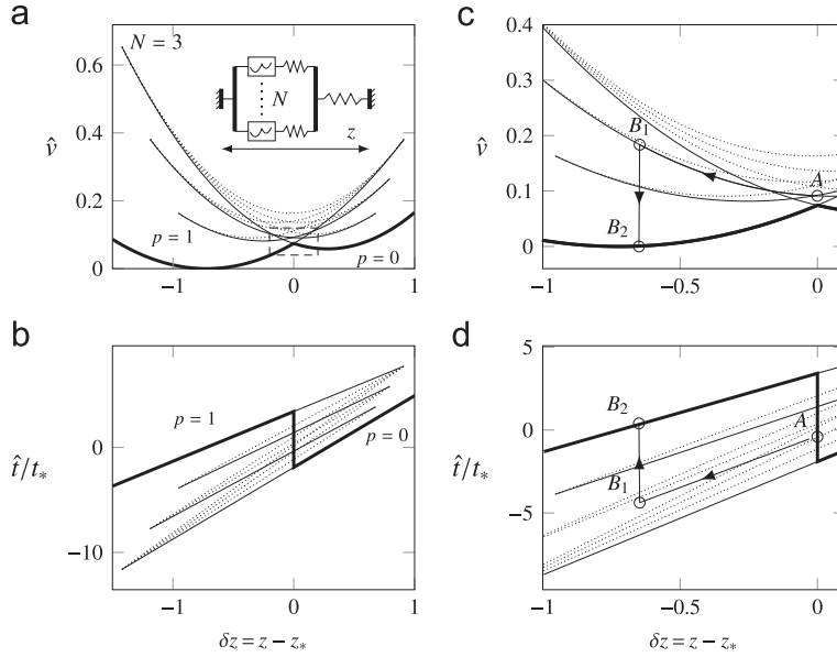
Fig. 9. Mechanical response of the snap-spring model in a hard device. (a) Energy levels of all the (p, q, r) configurations for the case N=3 at different applied elongations. (b) Corresponding tension–elongation relations. Solid lines, metastable states with p = 0, 1/3, 2/3, 1 and r = 1 - p, q = 0 ; dotted lines, unstable states with q \neq 0 ; thick lines, global minimum corresponding to p = 0, r = 1 , for z > z_* , and to p = 1, r = 0 , for z < z_* . (c and d) Blow-up of (a and b) illustrating the response of the system to abrupt shortening with an elastic unloading ( A \rightarrow B_1 ) followed by a massive conformational change in isometric conditions ( B_1 \rightarrow B_2 ). Parameters are \lambda_1 = 0.4, \lambda_0 = 0.7, l = -0.3, \lambda_b = 1 , and N=3 .
