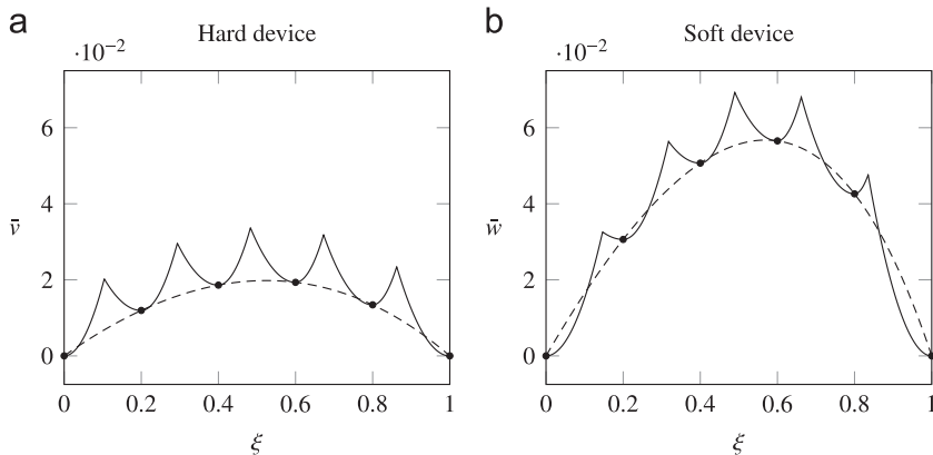
Fig. 11. Energy landscape at the global minimum transition for the snap-spring model with N=5 . (a) Hard device at z = z_* ; (b) soft device at t = t_* . Solid lines, successive barriers obtained from Eqs. (26) (a) and (31)(b); dashed lines, continuum limit, N \rightarrow \infty . Energy minima are arbitrarily set to 0 for comparison. Here, \lambda_b = 1 and other parameters are as in Fig. 9. In particular, we have \lambda_0 \neq \lambda_1 which explains why the curve is not symmetric.
