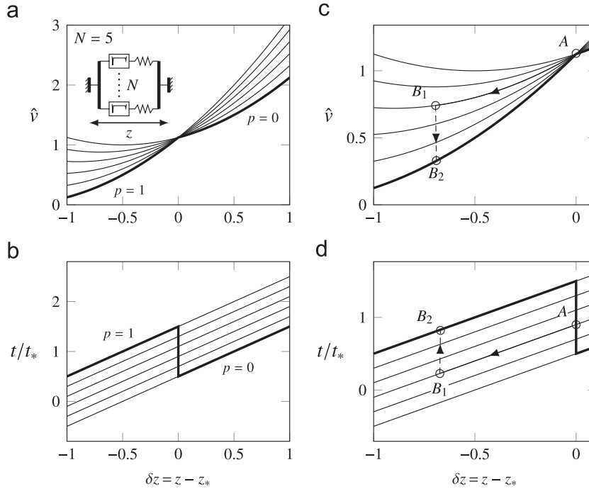
Fig. 3. Mechanical response of the HS model in a hard device with N=5 . (a) Energy levels of the metastable states ( p = 0, \frac{1}{5}, \dots, 1 ) for different applied elongations. (b) Corresponding tension–elongation relations. (c) and (d) are details of (a) and (b) with an illustrated response path to a fast loading experiment including a frozen elastic phase ( A \rightarrow B_1 ) followed by a subsequent phase equilibration ( B_1 \rightarrow B_2 ). Thick lines, global minimum corresponding to p=0 (resp. p=1 ) for z > z_* (resp. z < z_* ). t_* = v_0 and z_* = v_0 - 1/2 . Parameters are v_0 = 1 and N=5 .
