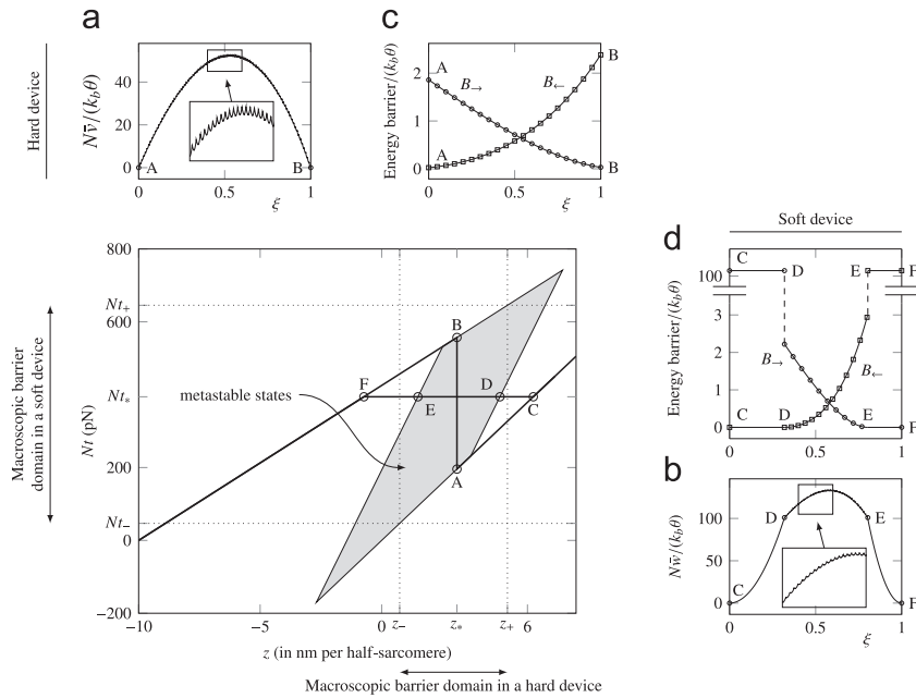
Fig. 14. Result of the soft spin model with parameters adjusted to fit experimental data, see Caruel et al. (2013). Main frame, tension–elongation relation for a single half-sarcomere. The gray area shows the existence domain of the metastable states. Solid lines, global minimum tension–elongation relation in hard and soft devices. (a) and (b) Energy landscape corresponding to single transition between the homogeneous states in a hard device ( A \rightarrow B ), see (a) and in a soft device ( C \rightarrow F ), see (b). (c) and (d) Size of the energy barriers corresponding to the individual folding ( B_{\rightarrow} ) and ( B_{\leftarrow} ) transitions obtained with both finite N (open symbols) and in the thermodynamic limit (solid lines). To improve readability of the finite N plots, we only show one out of five micro-transition points.
