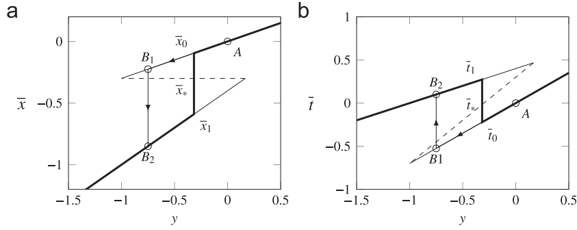
Fig. 8. Behavior of a single crosslinker in the snap-spring model. (a) Equilibrium positions for various y ; (b) corresponding tension levels. Solid lines, metastable states; dashed lines, unstable state; bold line, global minimum. Arrows indicate the response to a sudden shortening with an elastic unloading in the unfolded state ( A \rightarrow B_1 ) followed by the conformational change to the folded state ( B_1 \rightarrow B_2 ). Parameters are \lambda_1 = 0.4 , \lambda_0 = 0.7 , l = -0.3 .
