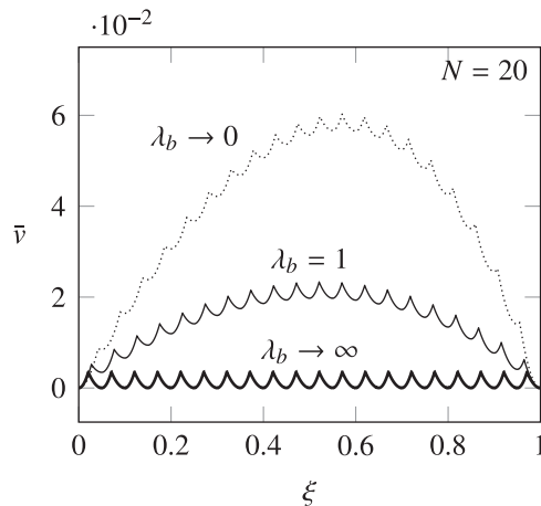
Fig. 12. Energy landscape at the global minimum transition for the snap-spring model in a hard device at different values of the coupling parameter \lambda_b with N=20 . Bold line, \lambda_b \rightarrow \infty ; solid line, \lambda_b = 1 ; dotted line, soft device limit as the hard device case where \lambda_b \rightarrow 0, z_* \rightarrow \infty . Energy minima are arbitrarily set to 0 for comparison. Other parameters are as in Fig. 9.
