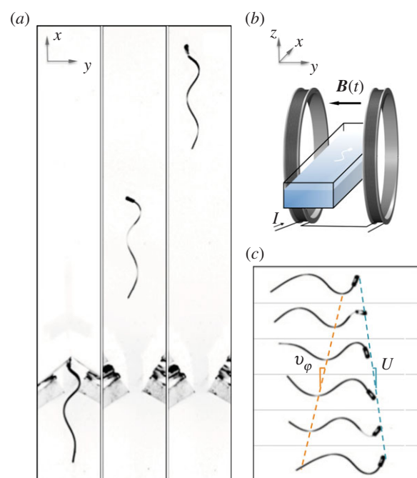
Figure 1. Experimental set-up: (a) Top-view snapshots of the swimmer propelling itself forward after the opening of the gates (that are visible at the bottom of the images). (See the electronic supplementary materials, movie S1, seeding particles have been added on the surface to visualize the flow.) (b) Swimmer at the free surface of a water tank consisting of a flexible cylindrical tail made of acrylic polymer. A magnet embedded in the head of the filament is forced to oscillate using the time-varying magnetic field produced by a Helmholtz pair. (c) Successive pictures of a filament over a period of undulation showing the forward swimming velocity, U , and the speed of the travelling wave, v_\varphi .
