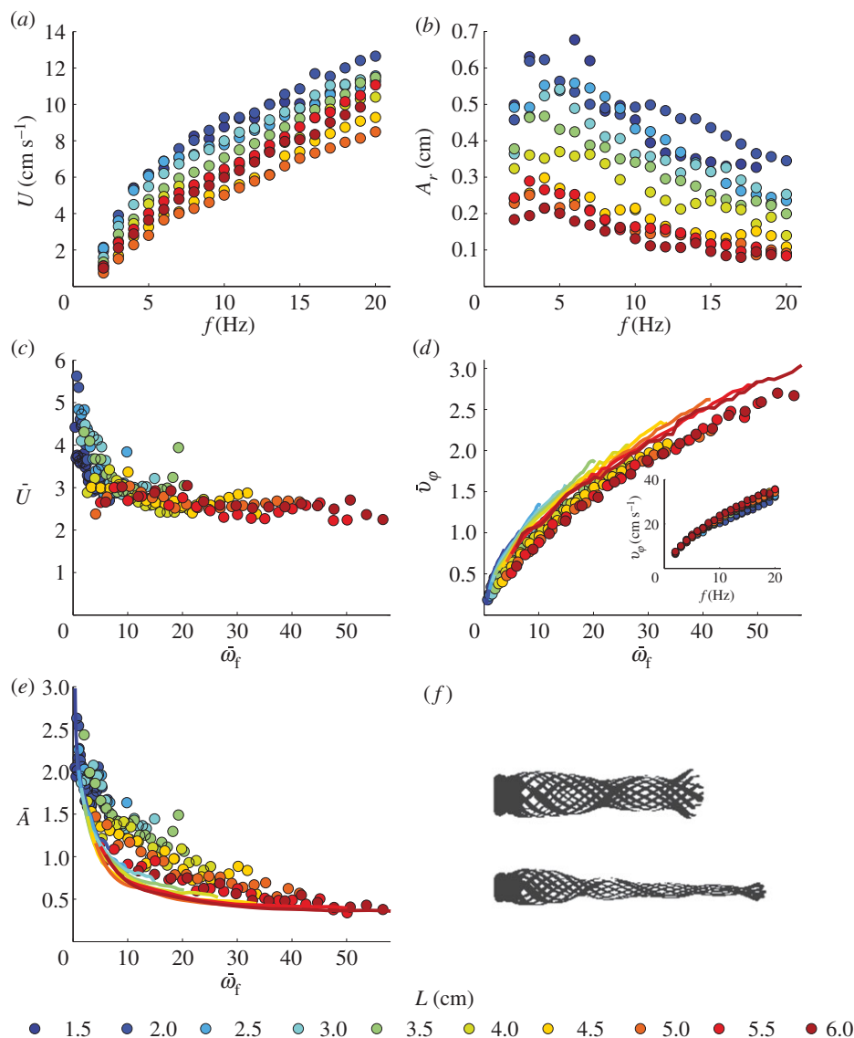
Figure 2. (a) Swimming velocity, (b) amplitude of the oscillations at the tail and (inset in d ) phase velocity, as a function of the forcing frequency. Experimental data plotted in a non-dimensionalized form, as a function of the non-dimensionalized angular frequency \tilde{\omega}_f = \omega_f/\omega_0 , with \omega_0 = (2\pi/L^2)(B/(\mu + \rho S))^{1/2} : (c) ratio of the cruising velocity and the characteristic actuation speed \bar{U} = U/fA_f , (d) non-dimensionalized phase velocity \bar{v}_\phi = v_\phi/\omega_0 L , (e) amplitude of the oscillation at the tail normalized by that of the head \bar{A} = A_r/A_f . The solid lines correspond to the theoretical predictions of the model presented in the ‘fluid–structure model’ section. (f) Typical undamped (3 cm long filament forced at 10 Hz) and damped (4 cm long filament forced at 20 Hz) amplitude envelopes (see the electronic supplementary material, movieS2 and S3).
