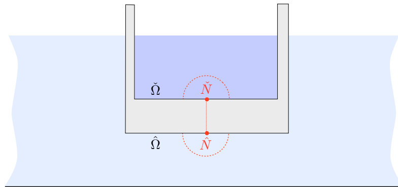
Figure A1. Mesoscopic regions \hat{\Omega} and \tilde{\Omega} . The jump on the potential \phi (or on the surface elevation \eta in (4)) is given at the mesoscopic scale and it corresponds to the dock problem on its own. The jump on the horizontal velocity \partial_x \phi (or on \partial_x \eta in (4)) is provided by zooming further in the vicinity of the points \hat{N} and \tilde{N} and within the neck \tilde{N}\hat{N} . This provides the microscopic problems which allows to connect the behaviors of the velocity potential \partial_x \phi inside and outside the resonant cavity.
