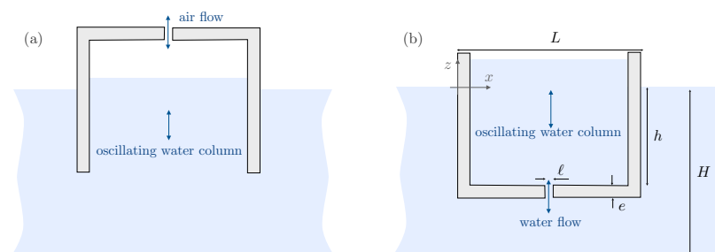
Figure 1. (a) Oscillatory water column (OWC); the power of the rising and falling water column is transferred to the air through a hole on the upper part of the cavity; the strong air flow is exploited by a power take off system [16]. (b) Helmholtz resonator with large oscillations of the water column due to strong water flow through a hole on the lower part of the cavity.
