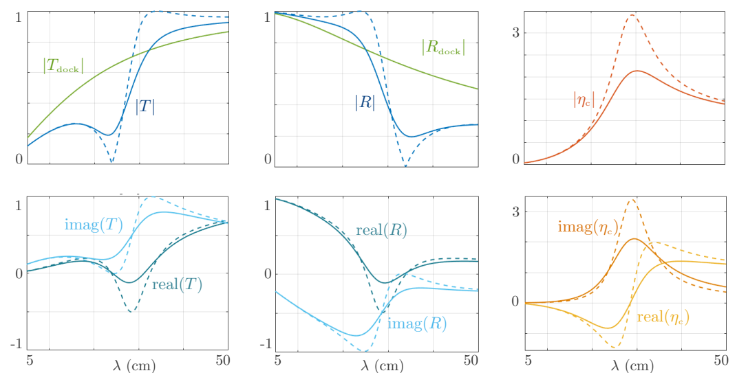
Figure 8. Predictions of the reduced model. Scattering coefficients (R, T) from (8) and amplitude \eta_c from (7) against the wavelength \lambda ; plain lines in the lossless case ( \sigma_L = 0 ) and dashed lines in the lossy case ( \sigma_L = 1.6 \text{ s}^{-1} ).
