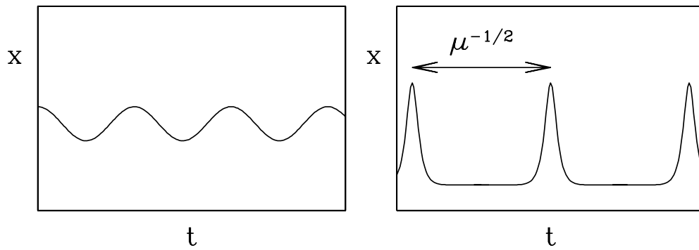
Figure 19: Timeseries during a limit cycle produced by a Hopf bifurcation (left) and a saddle-node bifurcation on a limit cycle (right), for parameter values near the bifurcation. The oscillation on the left is sinusoidal, whereas that on the right contains long phases during which the quantity plotted does not change, separated by short phases of sudden change.
