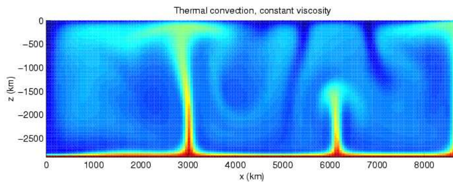
Figure 18: Numerical simulation of convection in the earth's mantle, containing plumes and thin boundary layers. By H. Schmeling, Wikimedia Commons. http://en.wikipedia.org/wiki/File:Convection-snapshot.gif
