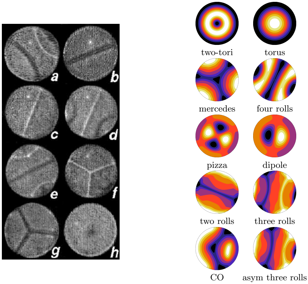
Figure 19: Left: experimental photographs of convection patterns in a cylindrical container whose radius is twice the height, all at the same Rayleigh number Ra = 14\,200 by Hof, Lucas, Mullin, Phys. Fluids 11 , 2815 (1999). Dark areas correspond to hot (rising) and bright to cold (descending) fluid. Right: numerical simulations by Borońska, Tuckerman, Phys. Rev. E (2010).
