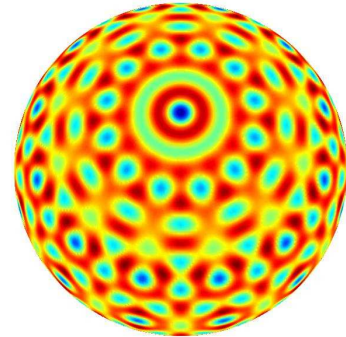
Figure 15: Convection pattern on sphere corresponding to spherical harmonic \ell = 28 , constructed by P. Matthews. From Phys. Rev. E . 67, 036206 (2003); Nonlinearity 16, 1449-1471 (2003);
