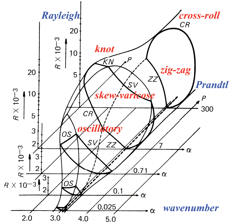
Figure 12: Instabilities of straight rolls. From Transition to Turbulence in Rayleigh-Bénard Convection by F.H. Busse. In Hydrodynamic Instabilities and the Transition to Turbulence ed. H.L. Swinney and J.P. Gollub, Springer 1981.
