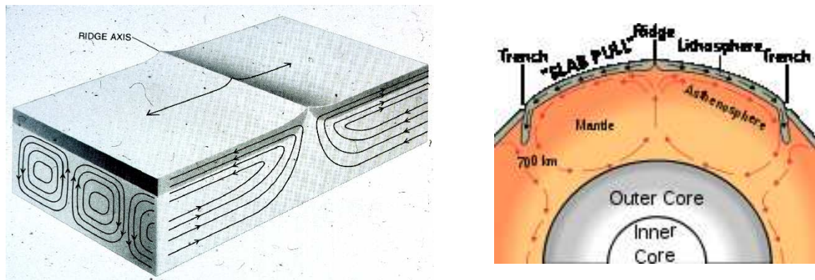
Figure 17: Convection and plate tectonics.
