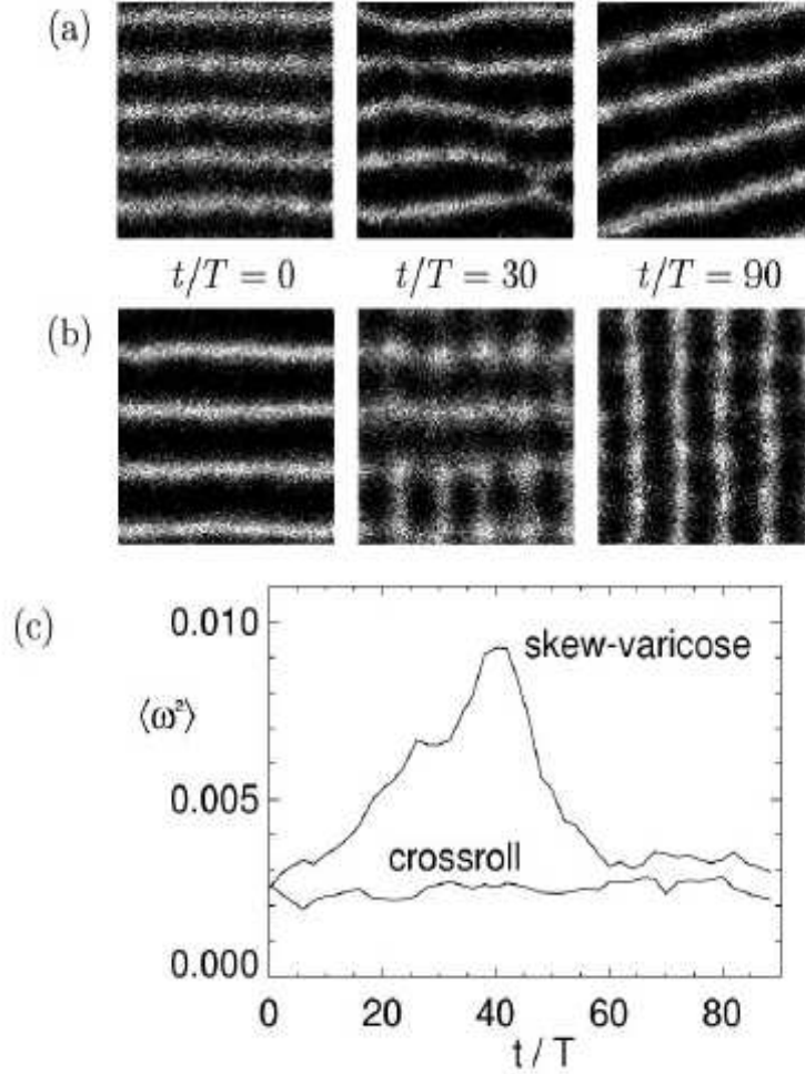
Figure 13: Instabilities of a striped pattern in a vertically-vibrated granular layer. Top: skew-varicose instability. Bottom: cross-roll instability. From J. de. Bruyn, C. Bizon, M.D. Shattuck, D. Goldman, J.B. Swift & H.L. Swinney, Continuum-type stability balloon in oscillated granulated layers , Phys. Rev. Lett. 81 , 1421 (1998).
