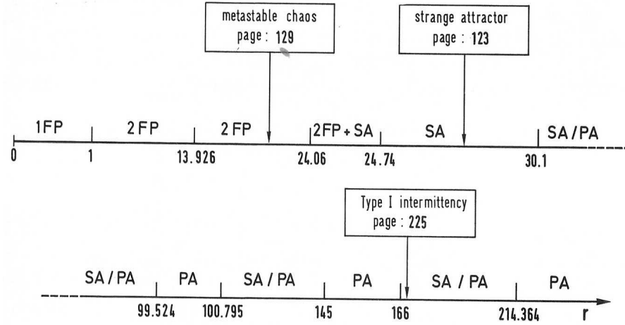
Figure 10: Regimes for the Lorenz model for r \lesssim 220 , showing ranges of existence of fixed points (FP), strange attractors (SA), and periodic attractors (PA). From Order within Chaos by P. Bergé, Y. Pomeau, C. Vidal, Wiley, 1986.
