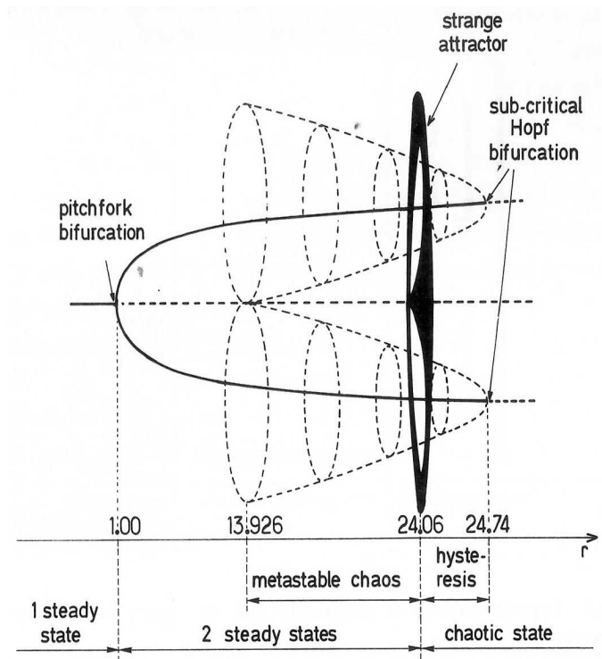
Figure 7: Bifurcation diagram for the Lorenz model for low r \lesssim 25 , showing supercritical pitchfork and subcritical Hopf bifurcations. From Order within Chaos by P. Bergé, Y. Pomeau, C. Vidal, Wiley, 1986.
