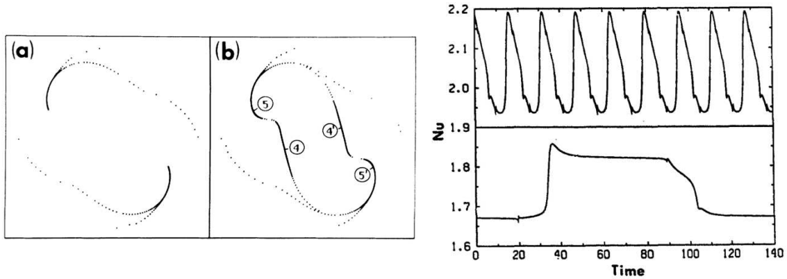
Figure 21: Left: phase portraits at Ra = 1.38Ra_c (left) and Ra = 1.39Ra_c (right).
