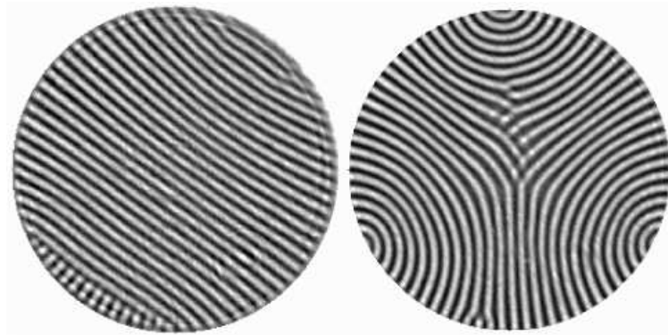
Figure 15: Convection pattern on sphere corresponding to spherical harmonic \ell = 28 , constructed by P. Matthews. From Phys. Rev. E . 67, 036206 (2003); Nonlinearity 16, 1449-1471 (2003);
