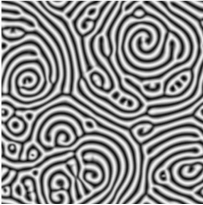
Figure 14: Spiral defect chaos in experimental convection. From Egolf, Melnikov, Pesche, Ecke, Nature 404 , 733-736 (2000).
