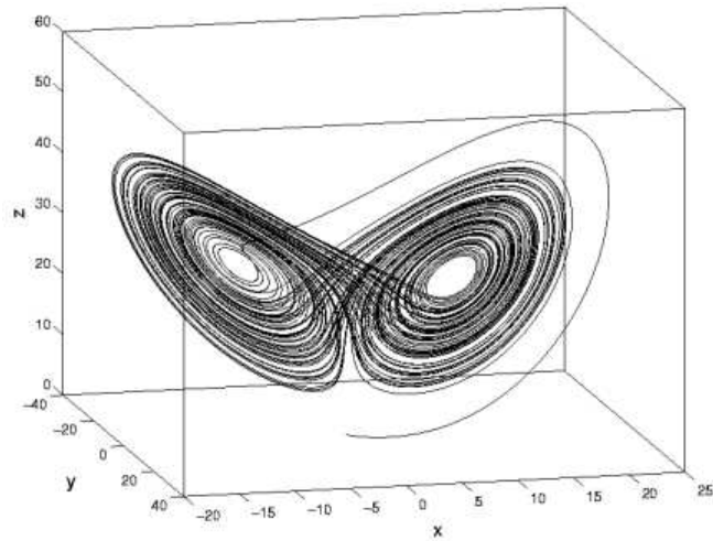
Figure 8: 3D view of chaotic Lorenz attractor at r = 28 .
