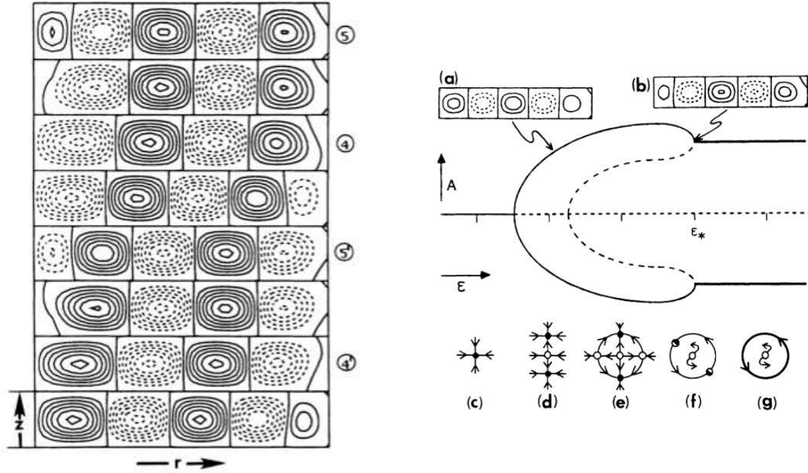
Figure 20: Left: (r, z) cut of toroidal convection cells in a cylindrical container whose radius is five times the height at Ra = 1.39Ra_c . The pattern moves radially inwards in time.
