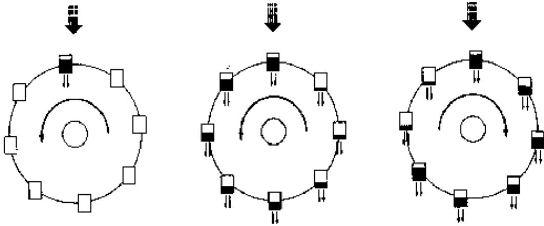
Figure 11: The Lorenz model does not provide a good description of Rayleigh-Bénard convection past threshold, but it does describe this waterwheel of leaking cups, proposed by W.V.R. Malkus.
