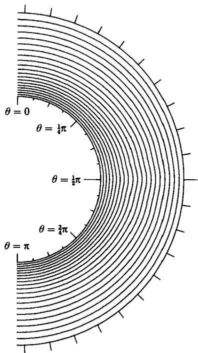
FIGURE 5. Contours of constant angular azimuthal velocity of the 0-vortex flow shown in figure 4. The tick marks and radial stretching are the same as those of figure 4. Except for a slight outward bulge at the equator due to the meridional outflow boundary, the angular velocity is approximately the Stokes flow and independent of \theta .
