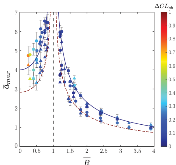
Fig. 2 Normalized maximal adhesion radius \bar{a}_{max} as a function of \bar{R} = R/\rho as predicted by eqn (2). Triangles (circles) correspond to caps deposited on the outer (inner) side of the rigid sphere, respectively. The color code represents the value of \Delta CL_{eb} for each data point. The data are well fitted by the asymptotic ( \Delta CL_{eb} = 0 ) theoretical law derived in the Appendix: \bar{a}_{max} = 4/\sqrt{1-\bar{R}^2} (blue solid line). The brown dashed line corresponds to the full law eqn (16) with \Delta CL_{eb} = 1 .
