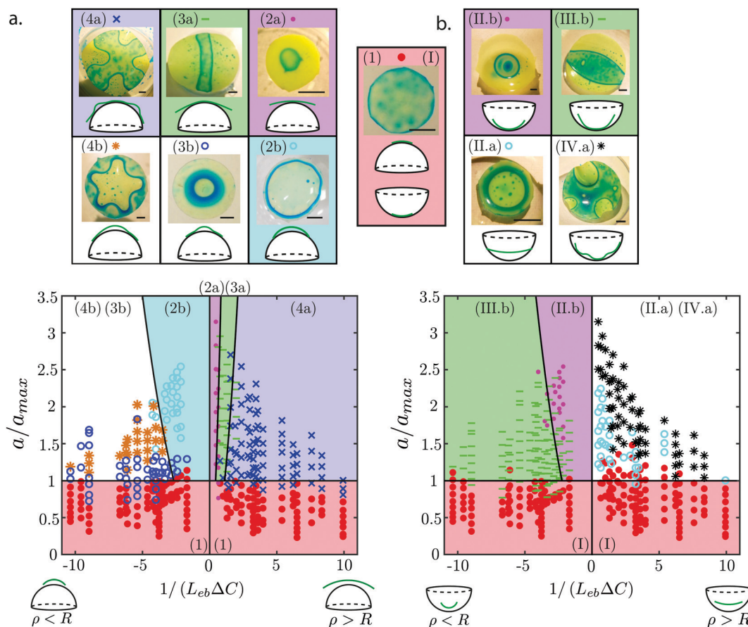
Fig. 3 Diagrams of configuration for the observed adhesion patterns when caps are put on the outside of spheres (a), and when caps are put inside of spheres (b). Different colors and symbols correspond to different patterns. Solid curved lines are scalings for boundaries between different adhesion patterns. Black bars on each picture are 1 cm.
