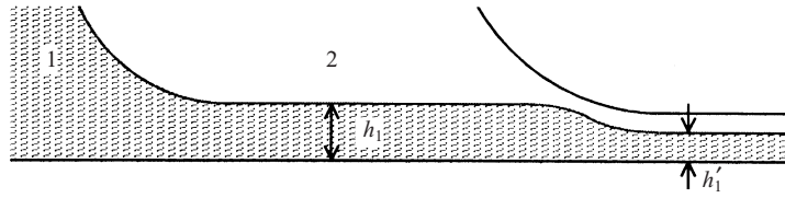
FIGURE 25. The two different thicknesses h_1 and h'_1 of the lubricant film.
