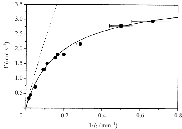
FIGURE 14. Velocity of an ethanol/silicone oil bislug in a dry polyethylene tube of radius 425\ \mu\text{m} with an ethanol index of constant length (13 mm). The data are compared with equation (12) (dotted line) and with a model taking into account additional dissipation in the menisci (equation (21), solid line).
