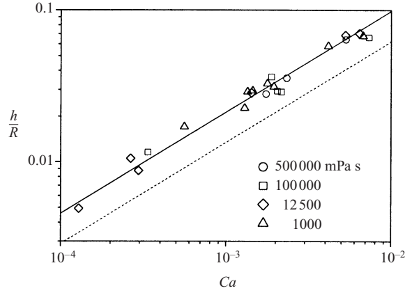
FIGURE 18. Lubricant film thickness measured for different oil viscosities and compared with the Schwartz–Bretherton law (equation (27), solid line) and with the Bretherton law (equation (17), dotted line).
