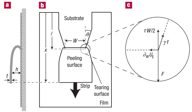
Figure 2 Schematic diagram showing the side and top views of the experiment and the geometrical parameters involved to describe the shape of the tear. a , Side view of the flap. The distance h gives the ‘height’ of the fold. b , Top view of the experiment. c , The close up shows a view of the tear at the position of the crack tip. The fracture propagation can be interpreted as the balance of four vectorial forces: two of them due to adhesion and fracture force, and the other two due to the pulling force and the inward force \partial_W U_E .
